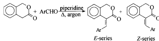
Scheme 2. Preparation of 4-(arylmethylene)-3-isochromanones 1–17
