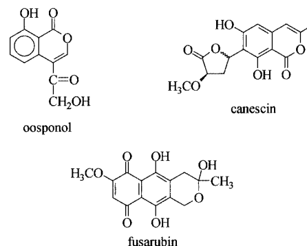
Scheme 1. Biologically important isochromane derivatives
