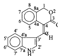
Scheme 3. Numbering of heavy atoms for NMR assignment of 14E
