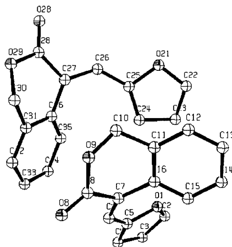
Figure 1. X-ray crystallography ORTEP diagram (30% thermal ellipsoids) showing the two rotamers in the unit cell of 13E
