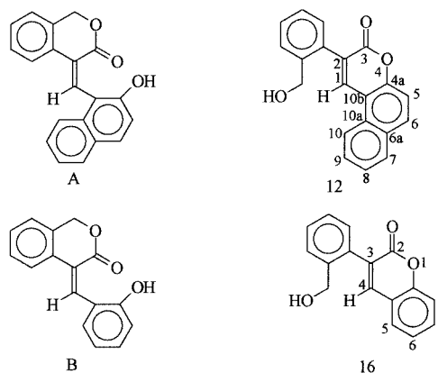
Scheme 4. Structures of coumarins ( 12 , 16 ) and the possible precursor isochromanones ( A , B )
